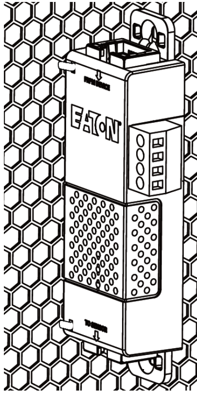
Side mounting
